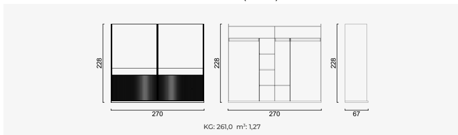
Wardrobe (Basic)
